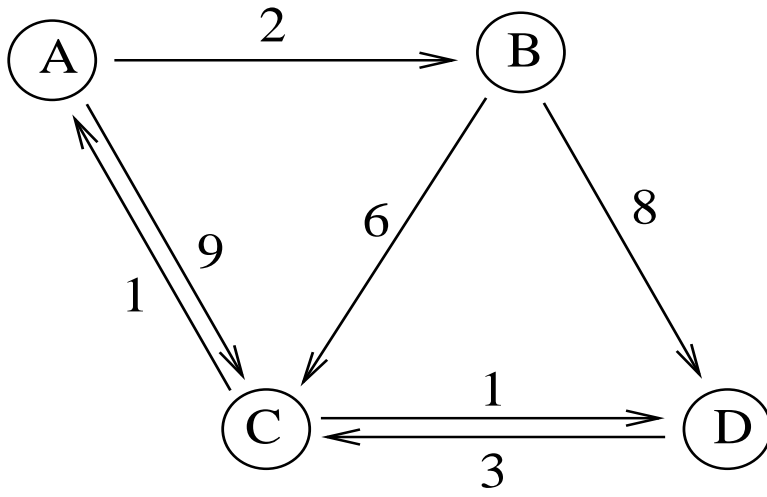
Figure 1: The weighted directed graph G .
