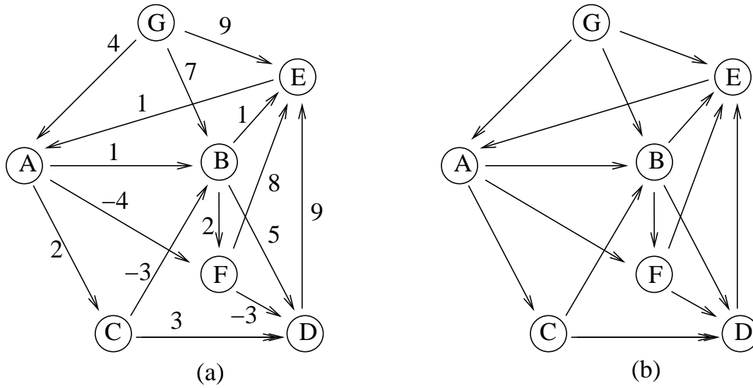
Figure 1: Place non-negative weights on graph (b) so that the new weighted graph is equivalent to the weighted graph in (a) for shortest path problems.
