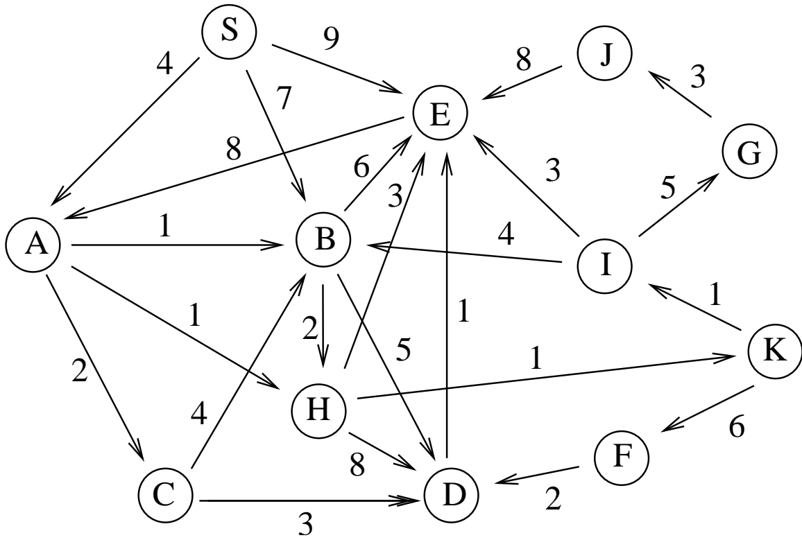
Figure 1: Use Dijkstra's Algorithm to solve the Single Source Minimum Path Problem
