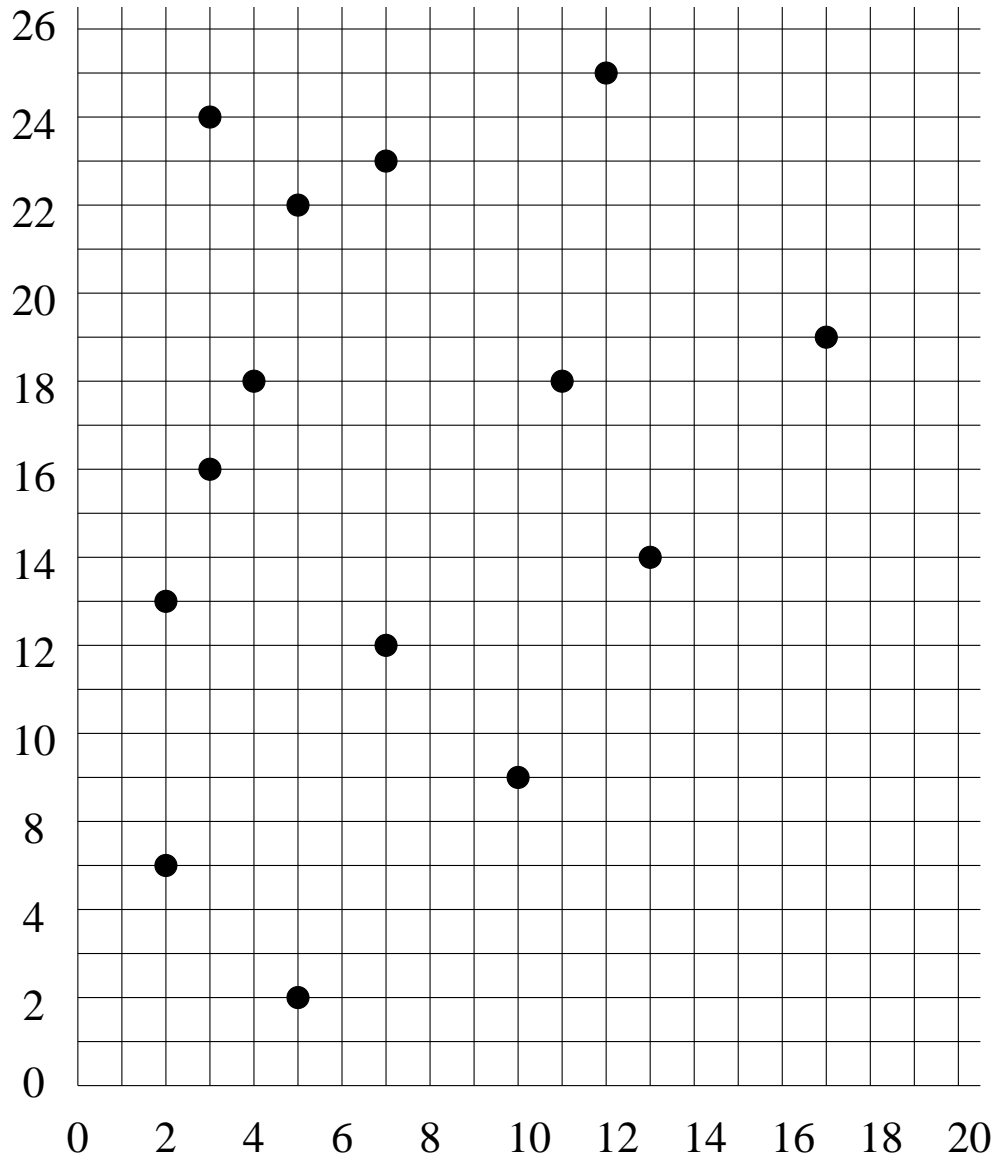
Figure 2: Use Graham's Scan to find the Convex Hull
