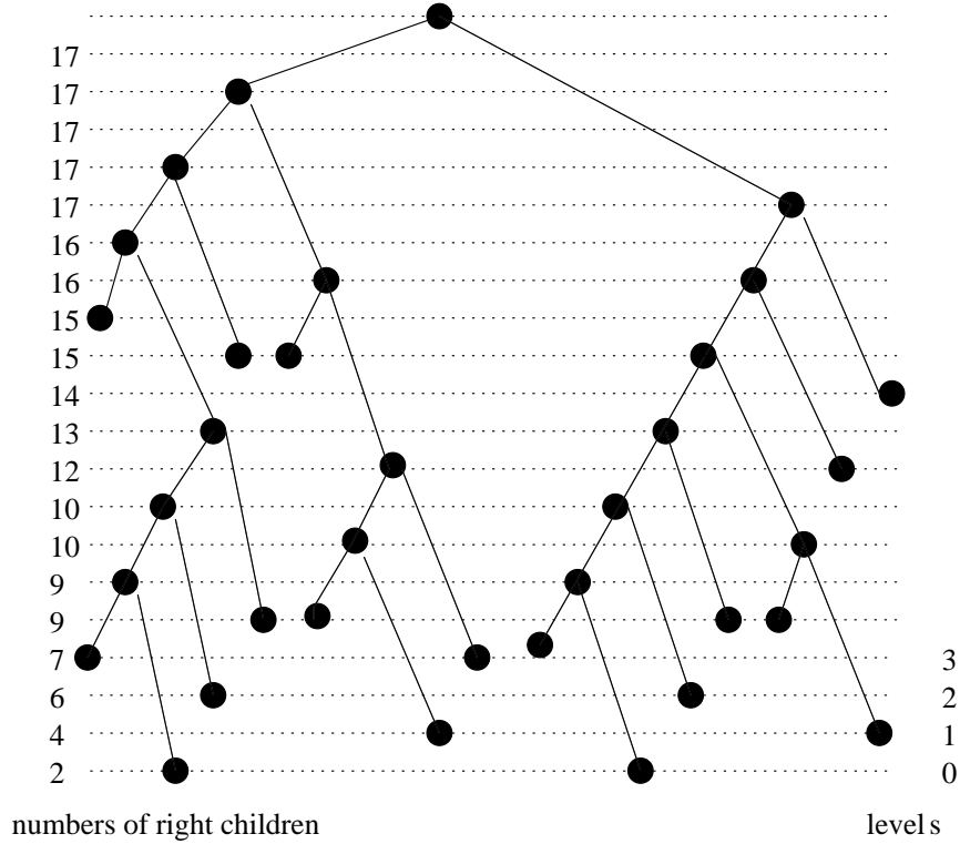
Figure 2: An 2-5 tree T with depth(T) = 20 and its characteristic sequence
