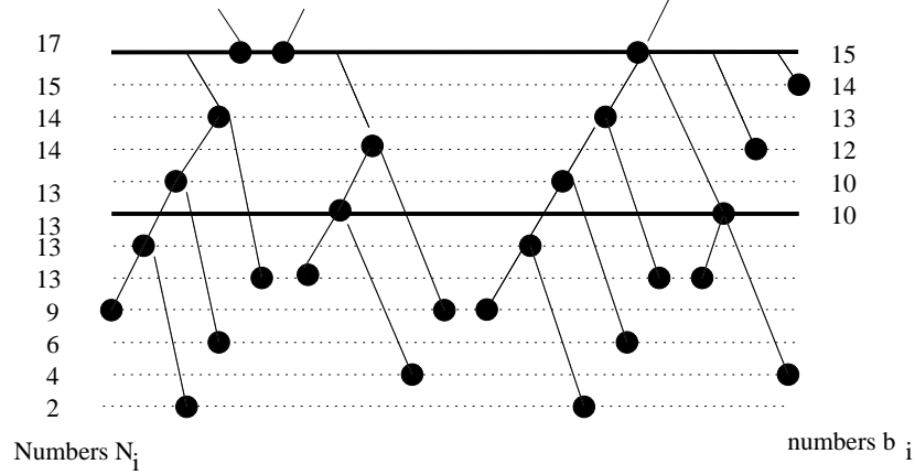
Figure 5: The bottom forest F_{11} of the tree T from Figure 2.
