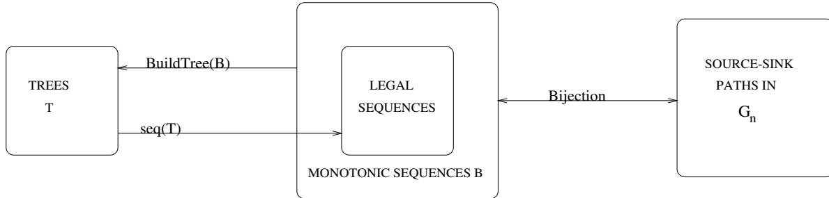
Figure 3: Relations between lopsided trees, monotonic sequences and graphs.
