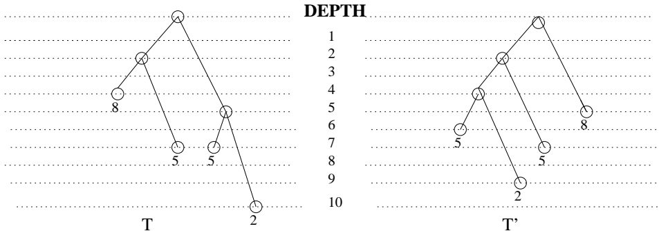
Figure 1: Two lopsided 2, 5 trees. The trees are labeled with P = \{2, 5, 5, 8\} .
