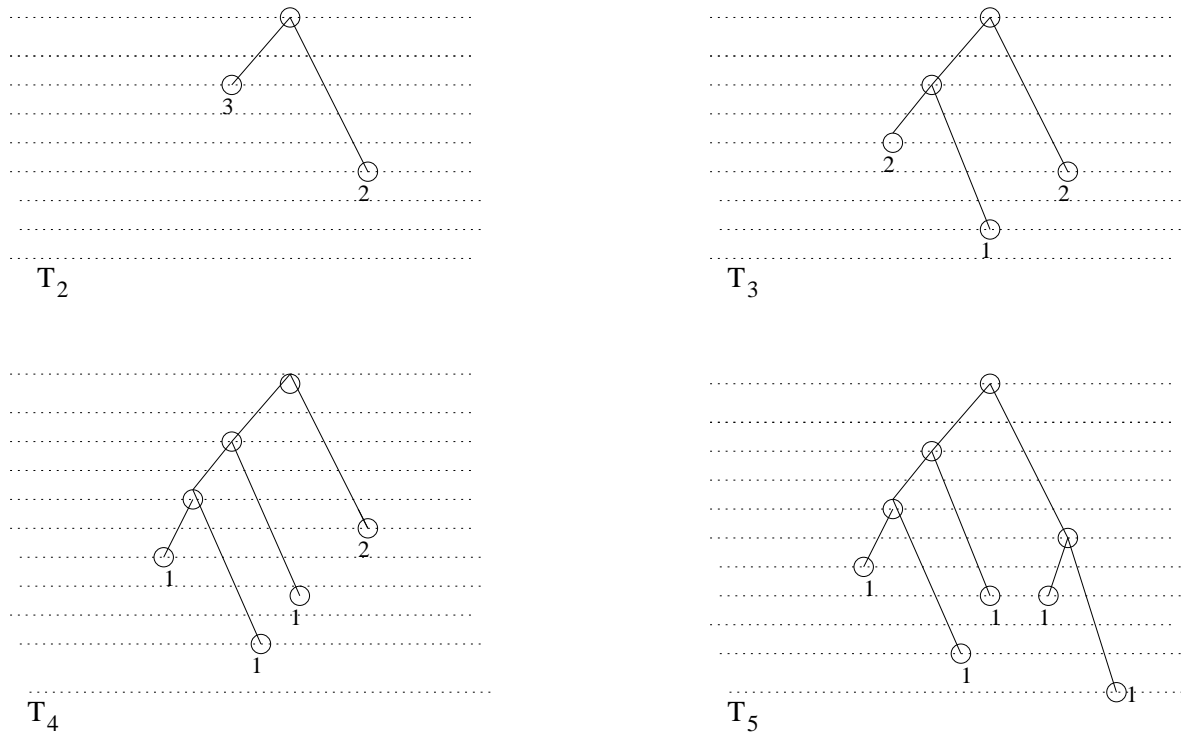
Figure 9: Trees generated by BuildTree(B_5) and its recursive calls. Tree T_i is labelled by P_i .
