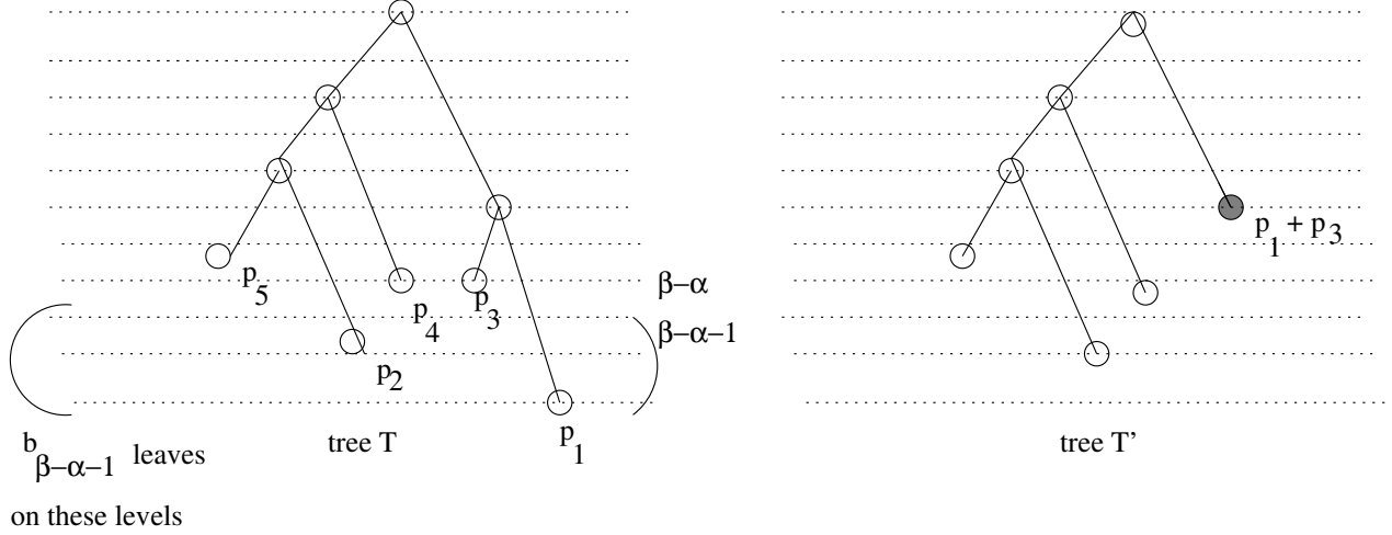
Figure 6: The correspondence between trees T , T' and their sequences: T' = \text{merge}(T, 1, 3) and \text{seq}(T) = B = (1, 2, 2, 3, 3, 4, 4, 4, 4, 4) ; \text{seq}(T') = \text{dec}(B) = B' = (0, 1, 1, 2, 2, 3, 3, 3, 3, 3) ; \text{FirstLeft}(B) = b_{\beta-\alpha-1} + 1 = b_{5-2-1} + 1 = 3 and \text{cost}(T) = \text{cost}(T') + 2p_4 + 5p_1 .
