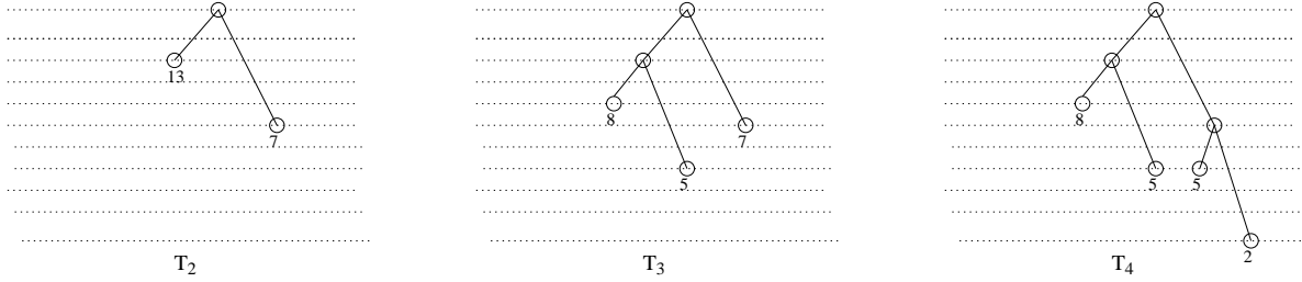
Figure 11: Trees generated by \text{BuildTree}(B_4) and its recursive calls. Tree T_i is labelled by P_i .
